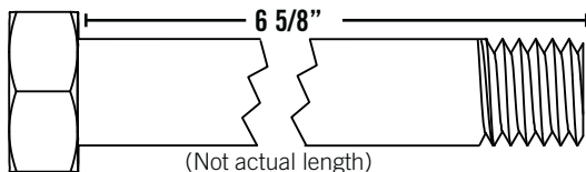
ADG (x4) 1/2" x 6 5/8" Hex Bolt
